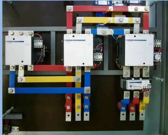
STAR DELTA
